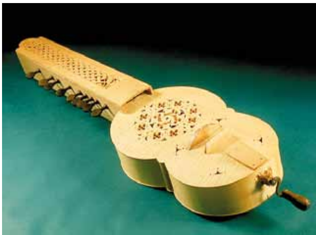
Organistrum
